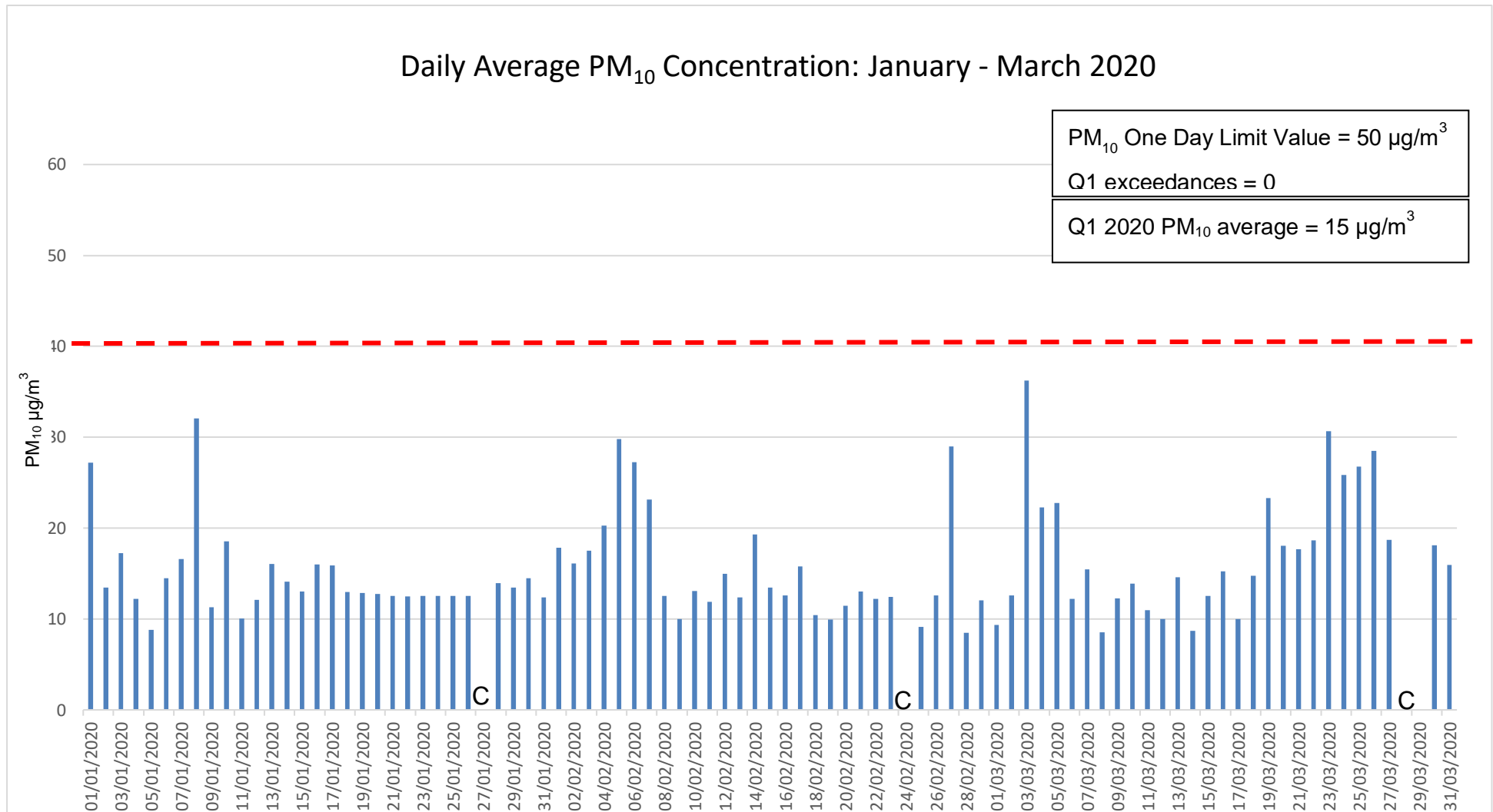
Figure 5 Daily Average PM 10 Q1 2020
