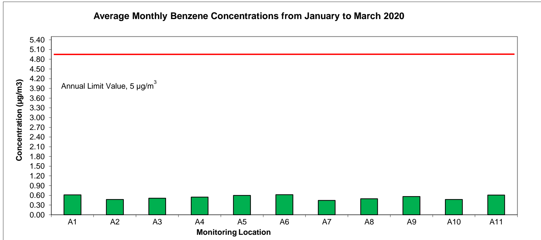
Figure 3 Average Monthly Benzene (C 6 H 6 ) Concentrations Q1 2020
