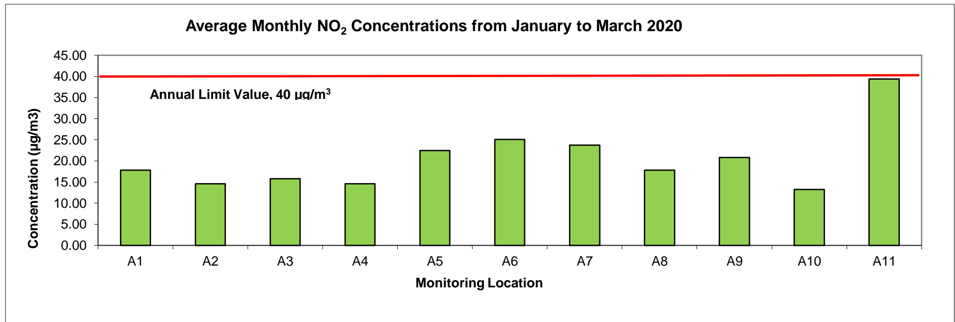
Figure 2 Average Monthly NO 2 Concentrations Q1 2020
