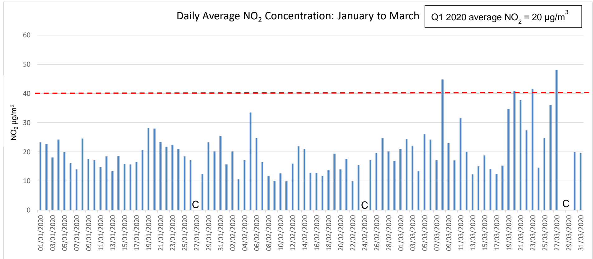
Figure 4 Daily Average NO 2 Q1 2020
