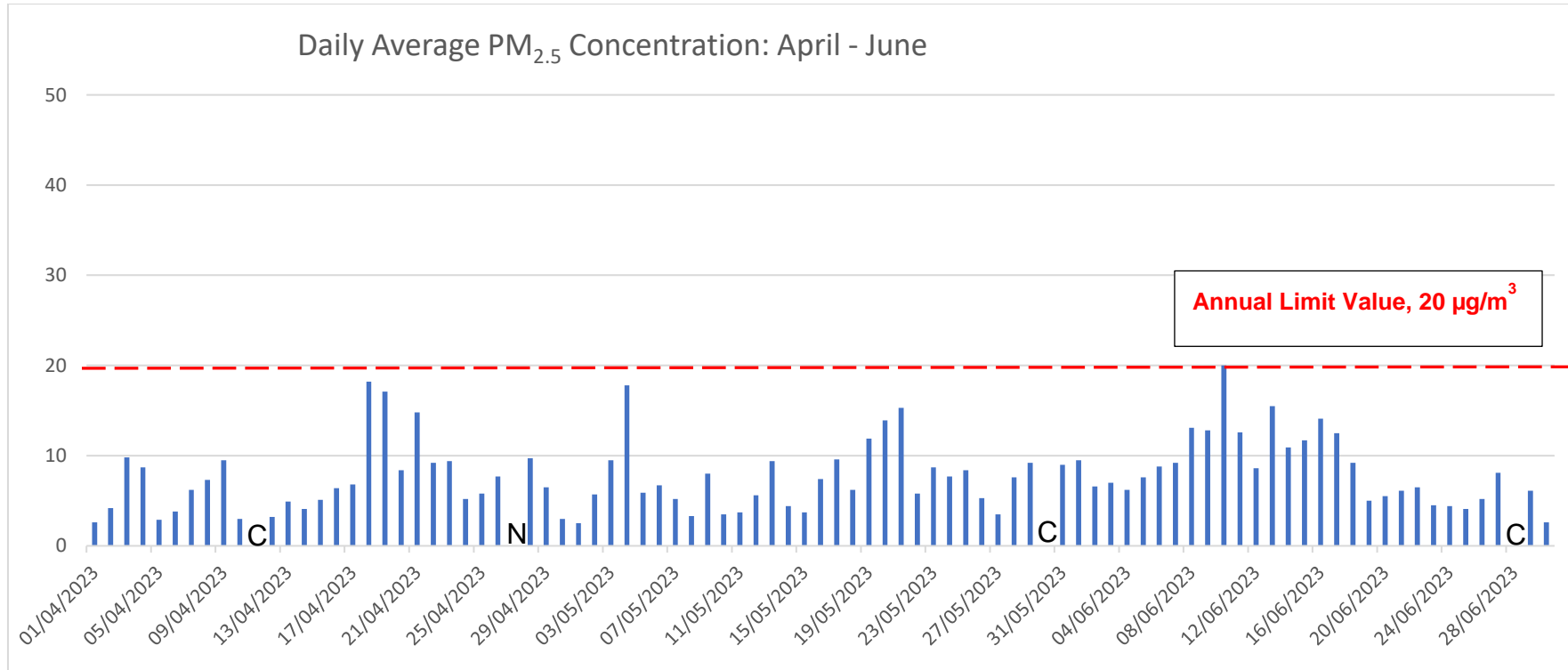
Figure 6 Daily Average PM 2.5 Q2 2023
