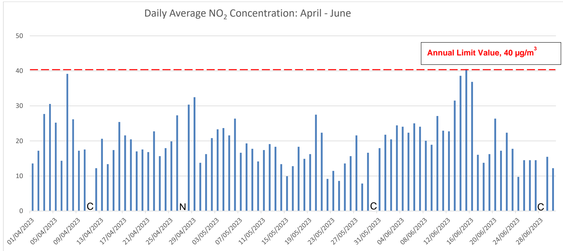
Figure 4 Daily Average NO 2 Q2 2023
