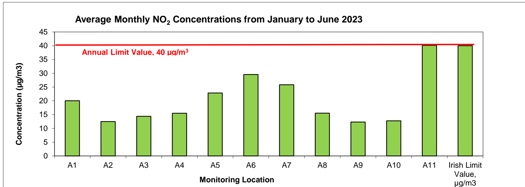
Figure 2 Average Monthly NO 2 Concentrations Q2 2023
