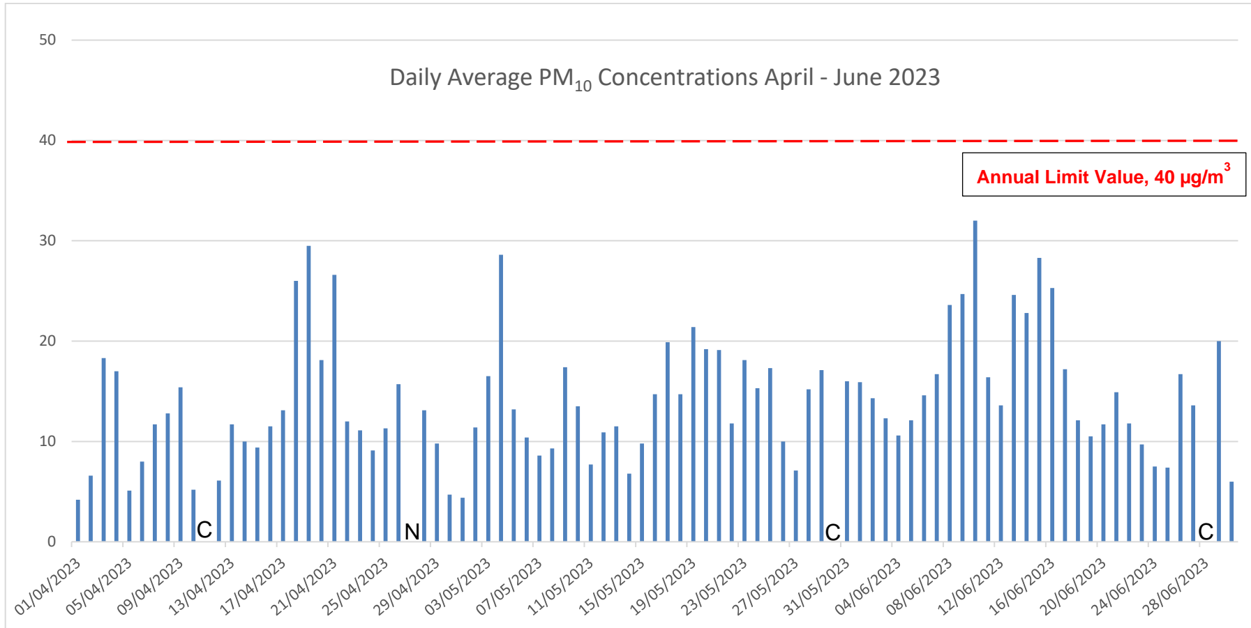
Figure 5 Daily Average PM 10 Q2 2023
