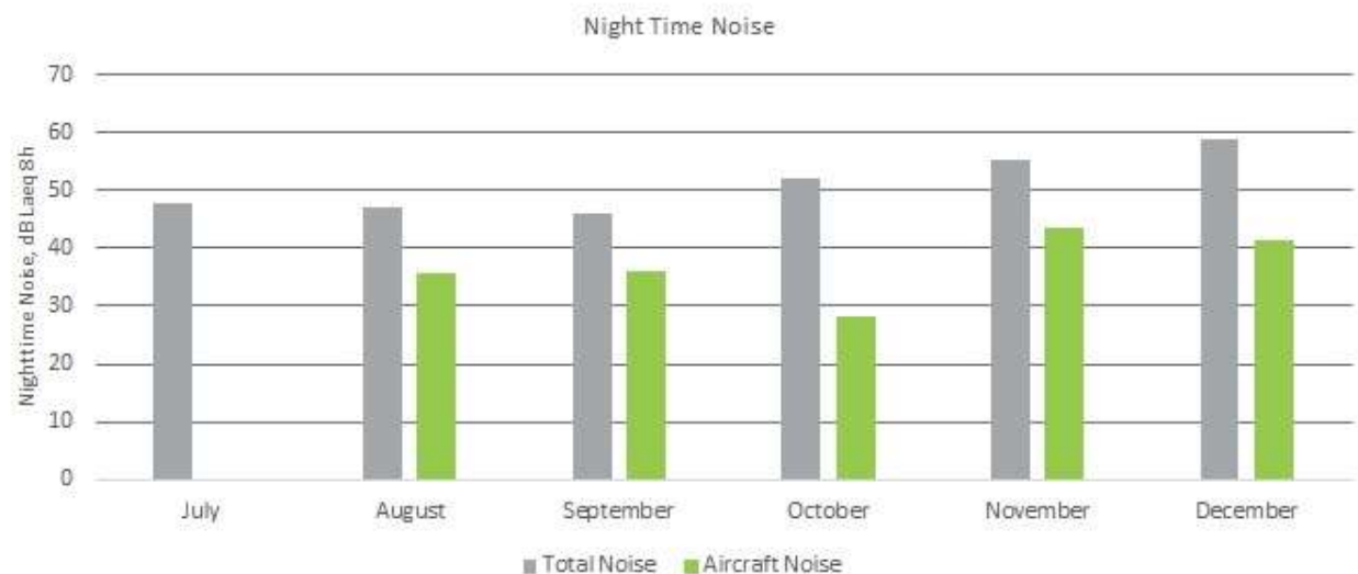
Figure 49: Averaged night-time noise levels for NMT 6, July - December 2021
