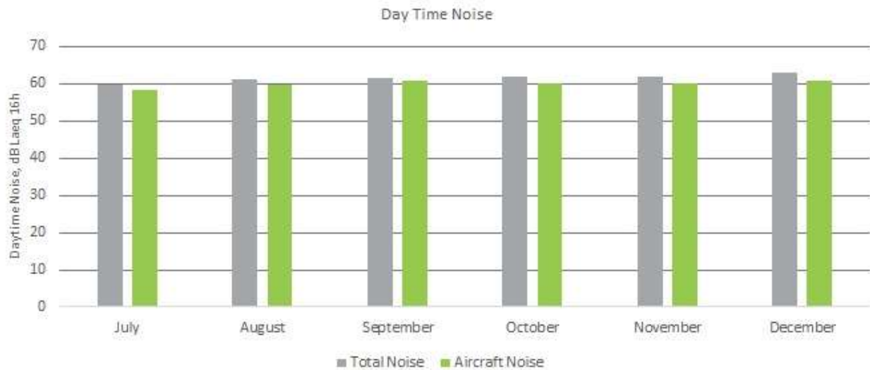
Figure 13: Averaged daytime noise levels for NMT 1, July - December 2021
