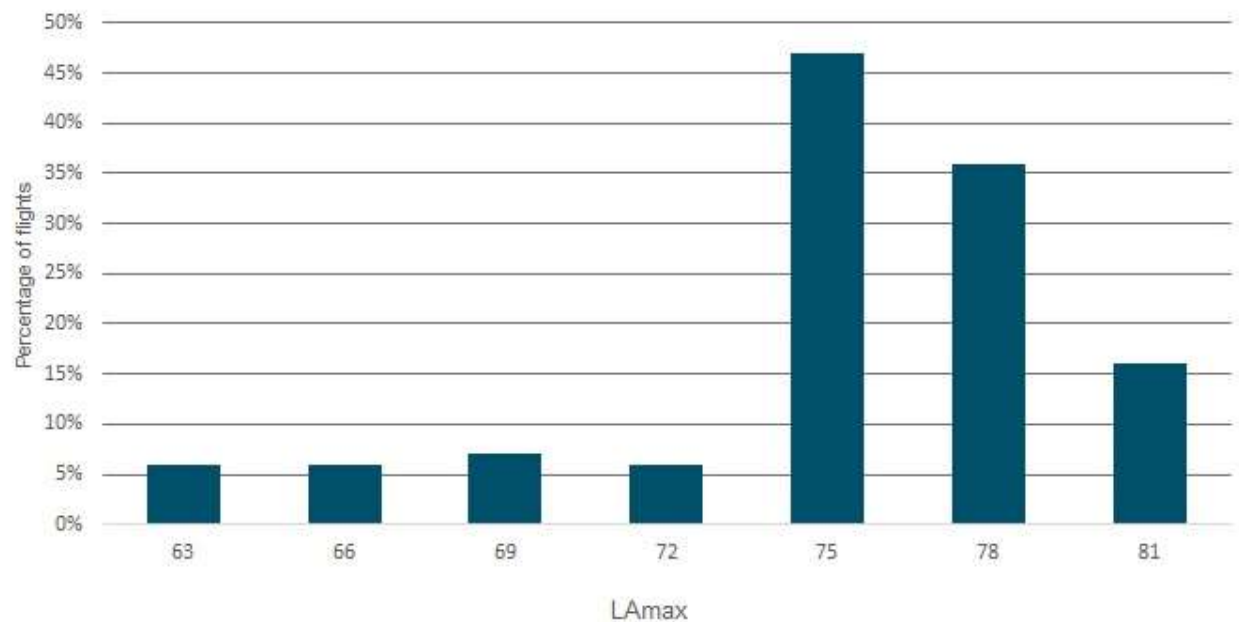
Figure 44: L Amax levels distribution for NMT 5, July - December 2021
