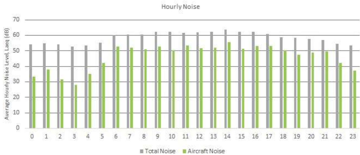
Figure 29: Averaged hourly noise levels for NMT 3, July - December 2021
