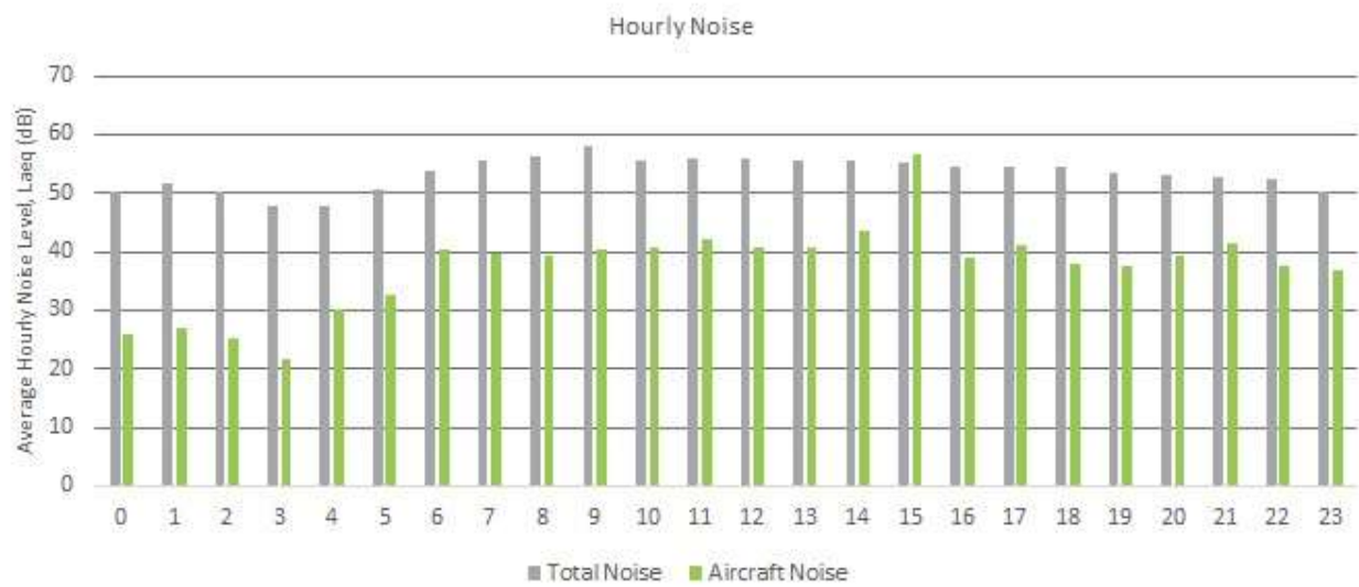
Figure 36: Averaged hourly noise levels for NMT 4, July - December 2021
