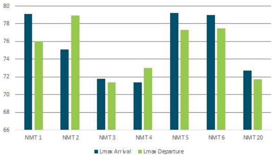
Figure 7: Average LAmax levels distribution for NMTs for arriving and departing aircraft, July - December 2021
