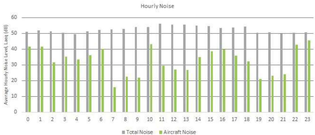
Figure 43: Averaged hourly noise levels for NMT 5, July - December 2021
