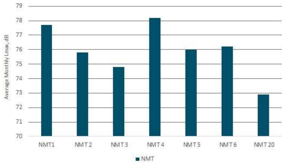
Figure 6: Average LAmax levels distribution for NMTs, July – December 2021
