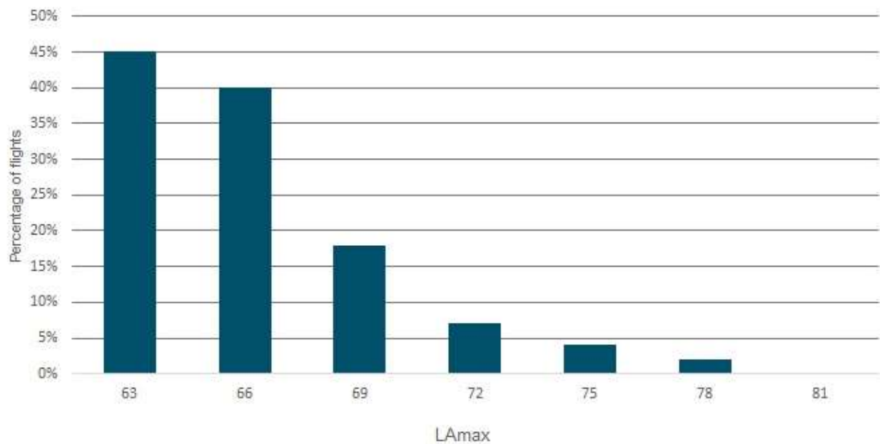
Figure 37: L Amax levels distribution for NMT 4, July - December 2021
