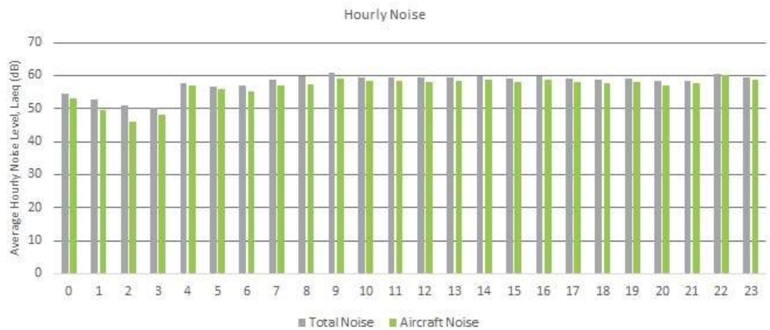
Figure 22: Averaged hourly noise levels for NMT 2, July - December 2021
