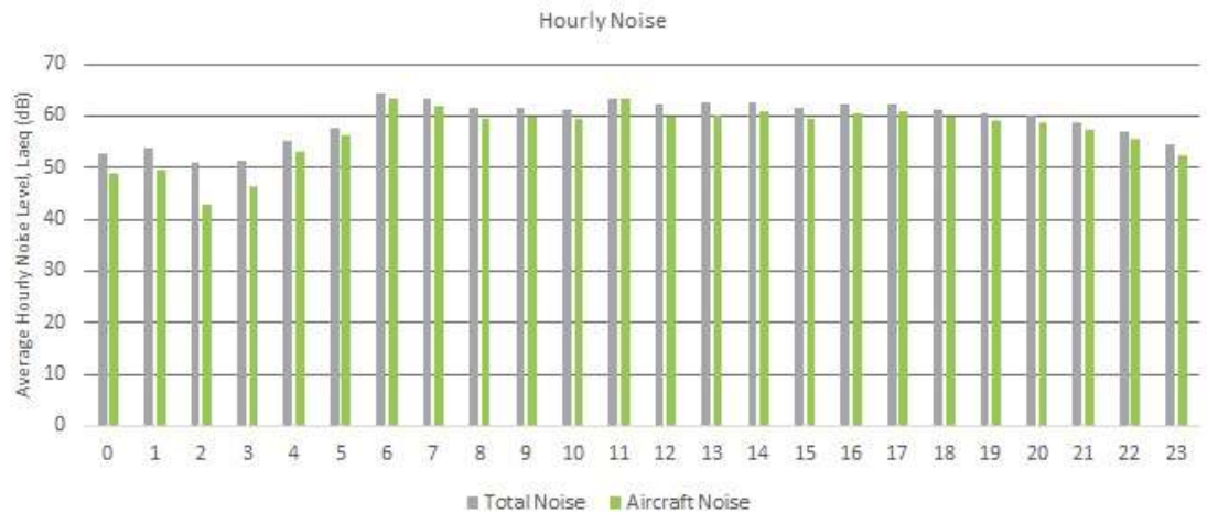
Figure 15: Averaged hourly noise levels for NMT 1, July - December 2021
