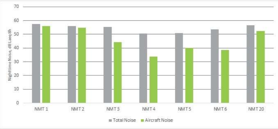
Figure 9: Averaged night-time noise levels per NMTs, July - December 2021
