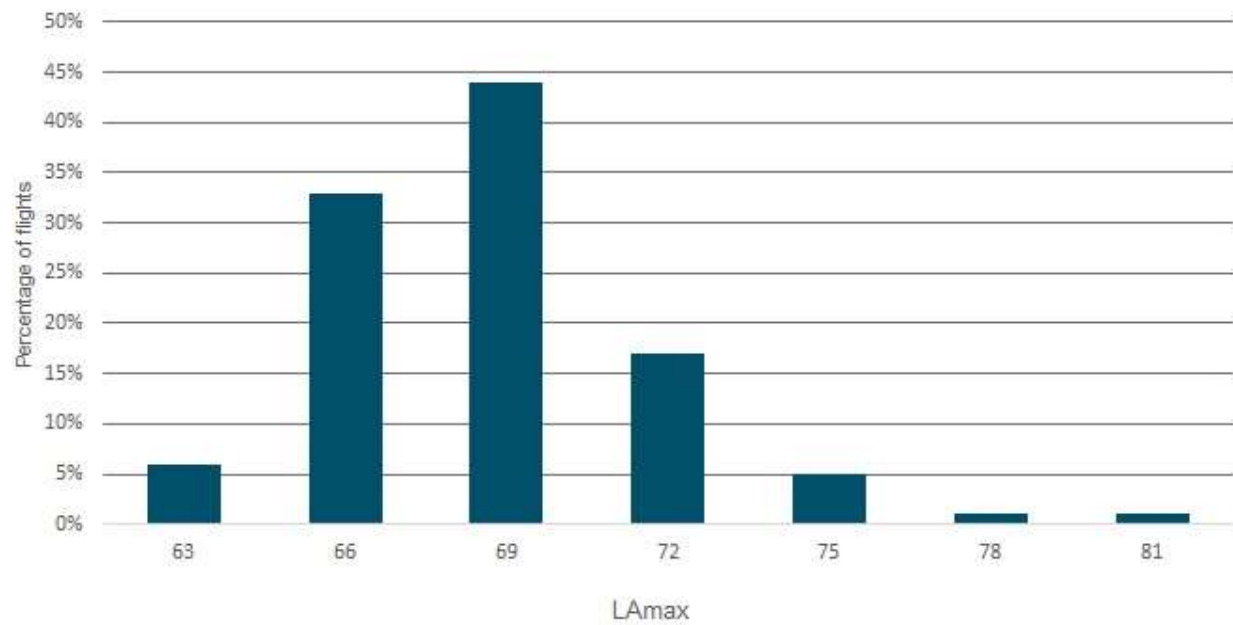
Figure 30: LAmax levels distribution for NMT 3, July - December 2021
