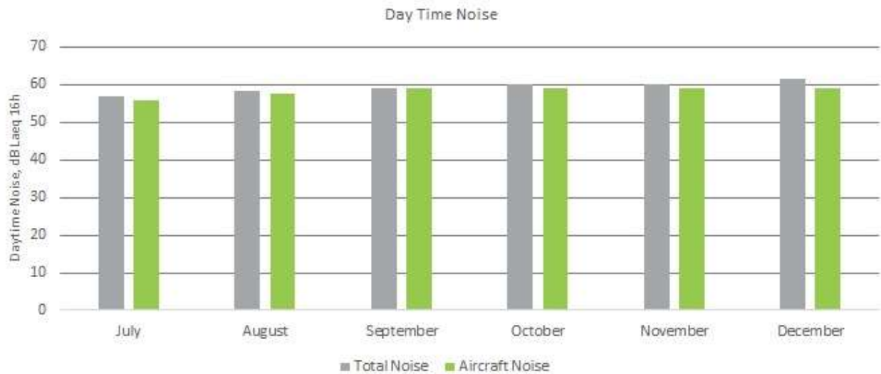
Figure 20: Averaged daytime noise levels for NMT 2, July - December 2021
