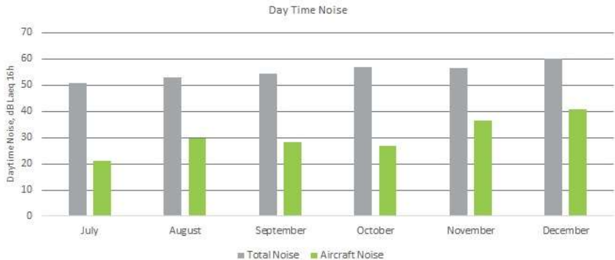
Figure 48: Averaged daytime noise levels for NMT 6, July - December 2021
