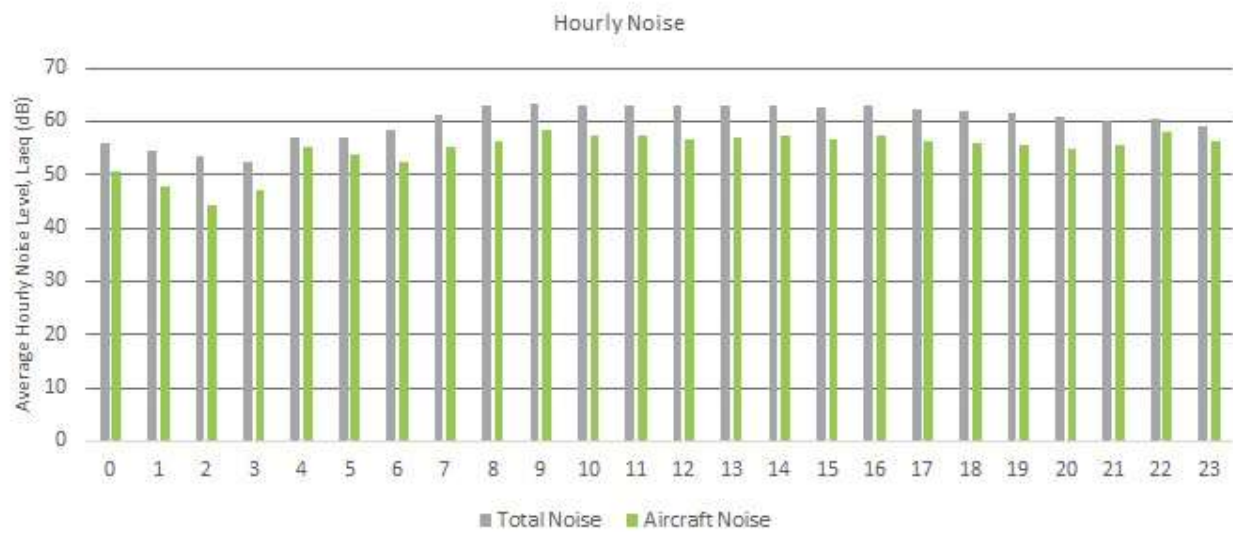
Figure 57: Averaged hourly noise levels for NMT 20, July - December 2021
