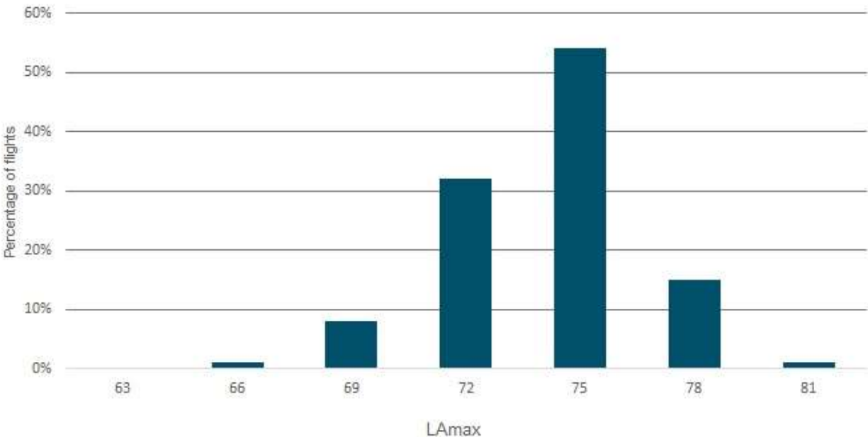
Figure 16: L_{Amax} levels distribution for NMT 1, July - December 2021
