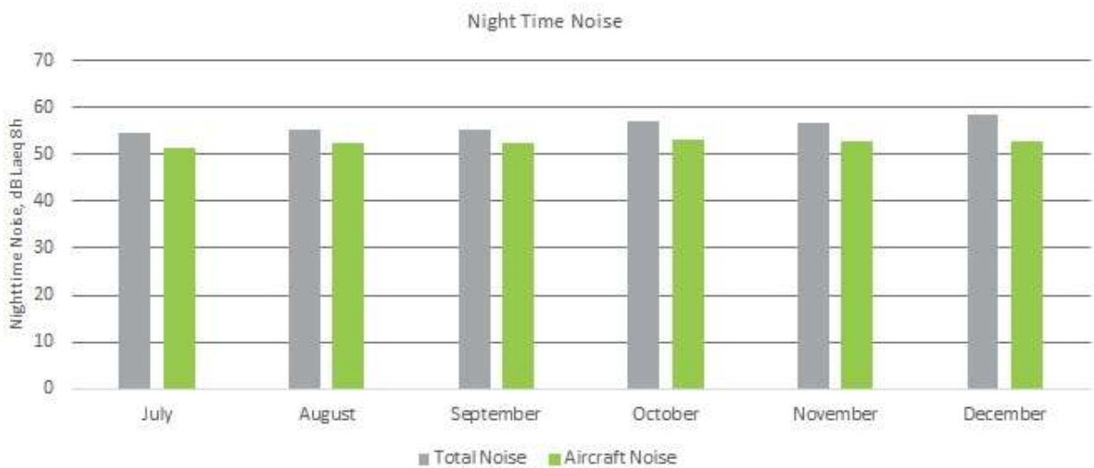
Figure 56: Averaged night-time noise levels for NMT 20, July - December 2021
