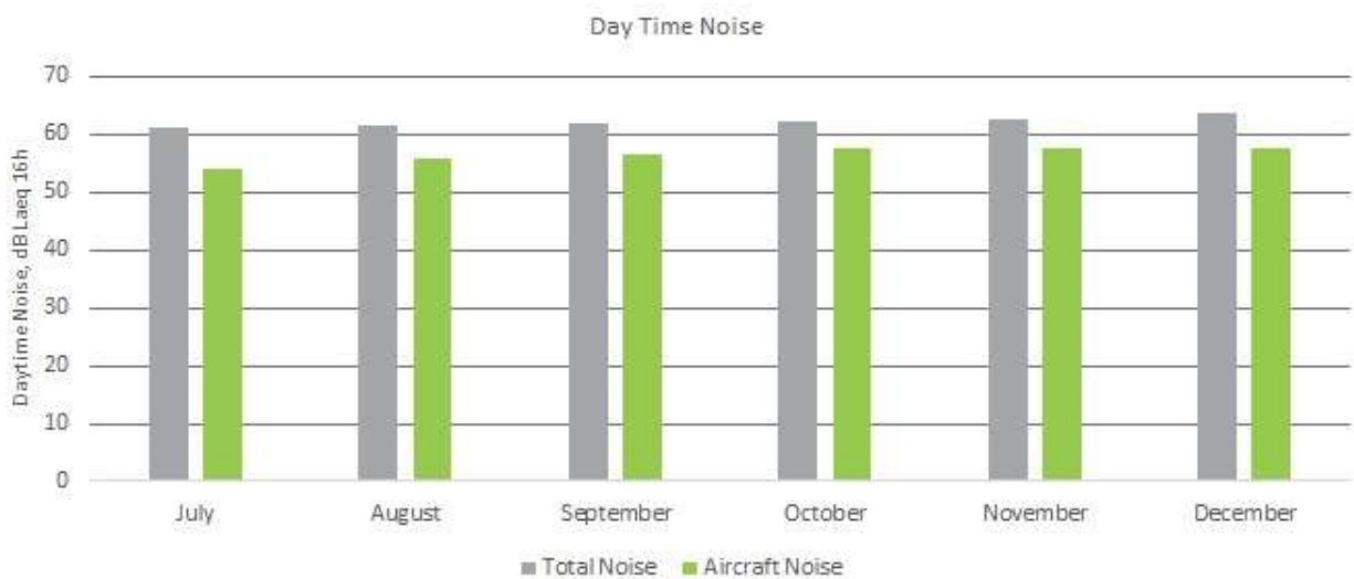
Figure 55: Averaged daytime noise levels for NMT 20, July - December 2021
