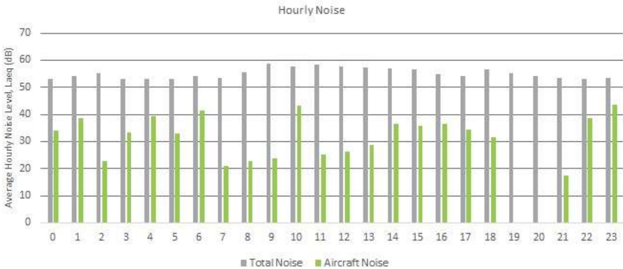
Figure 50: Averaged hourly noise levels for NMT 6, July - December 2021
