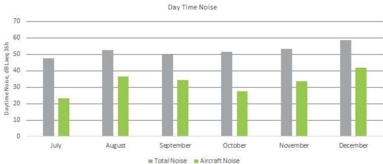
Figure 41: Averaged daytime noise levels for NMT 5, July - December 2021
