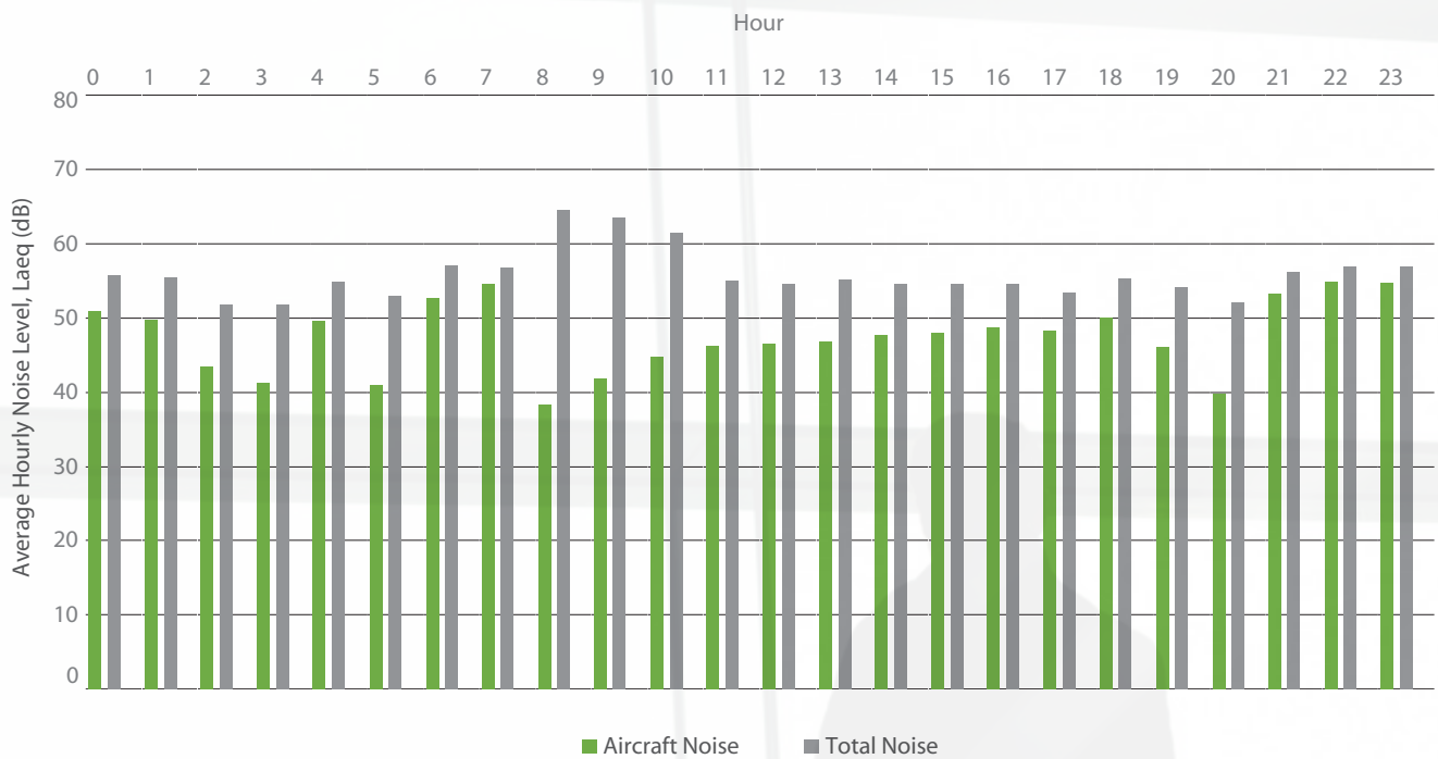
Figure 32: Averaged hourly noise levels for NMT 5, January - June 2018
