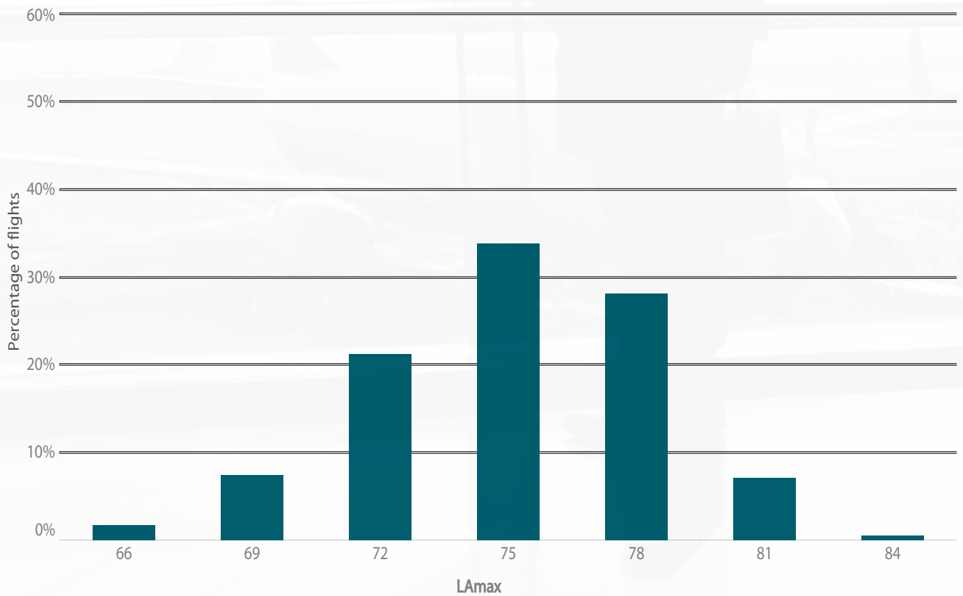
Figure 12: L_{A,MAX} levels distribution for NMT 1, January - June 2018
