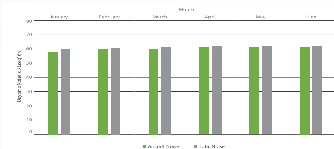
Figure 16: Averaged daytime noise levels for NMT 2, January - June 2018
