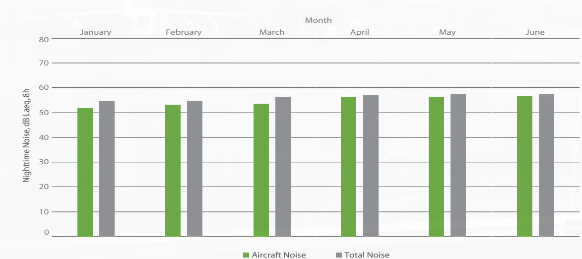
Figure 17: Averaged nighttime noise levels for NMT 2, January - June 2018
