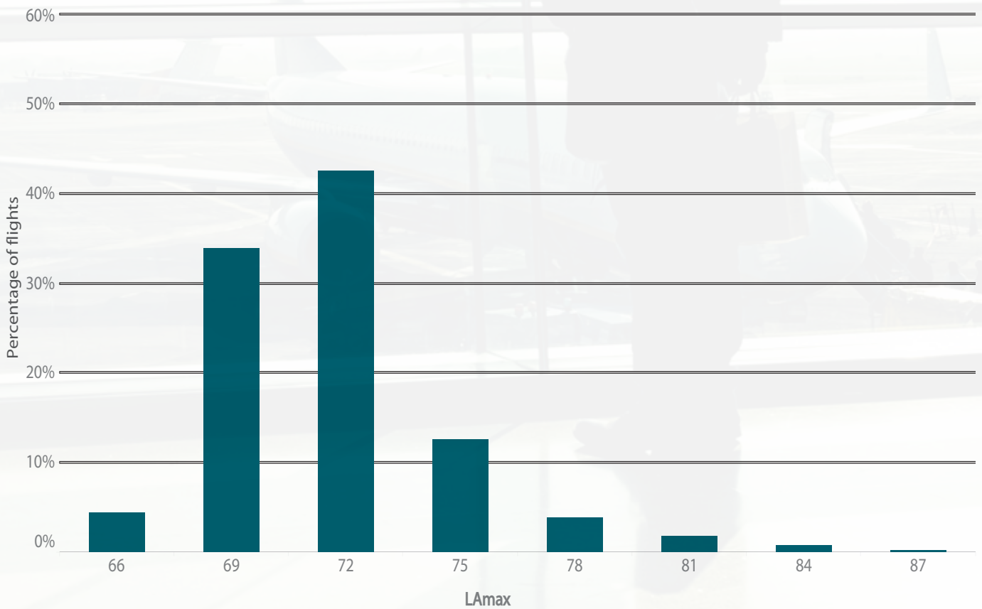
Figure 47: L_{A,MAX} levels distribution for NMT 20, January - June 2018
