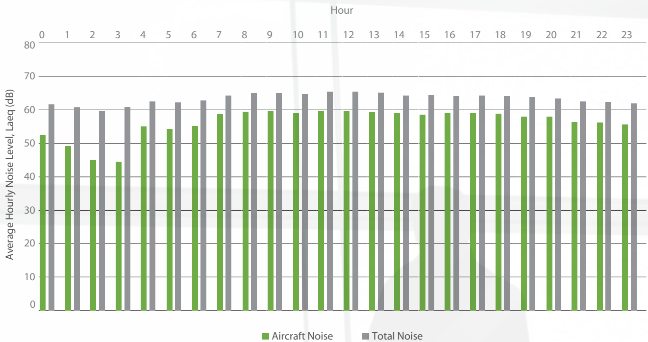
Figure 46: Averaged hourly noise levels for NMT 20, January - June 2018
