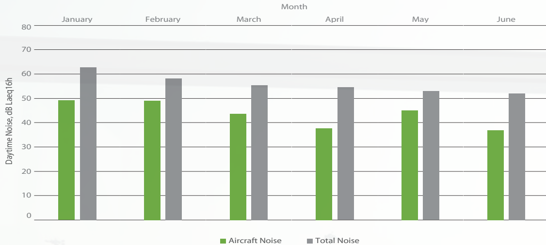
Figure 37: Averaged daytime noise levels for NMT 6, January - June 2018
