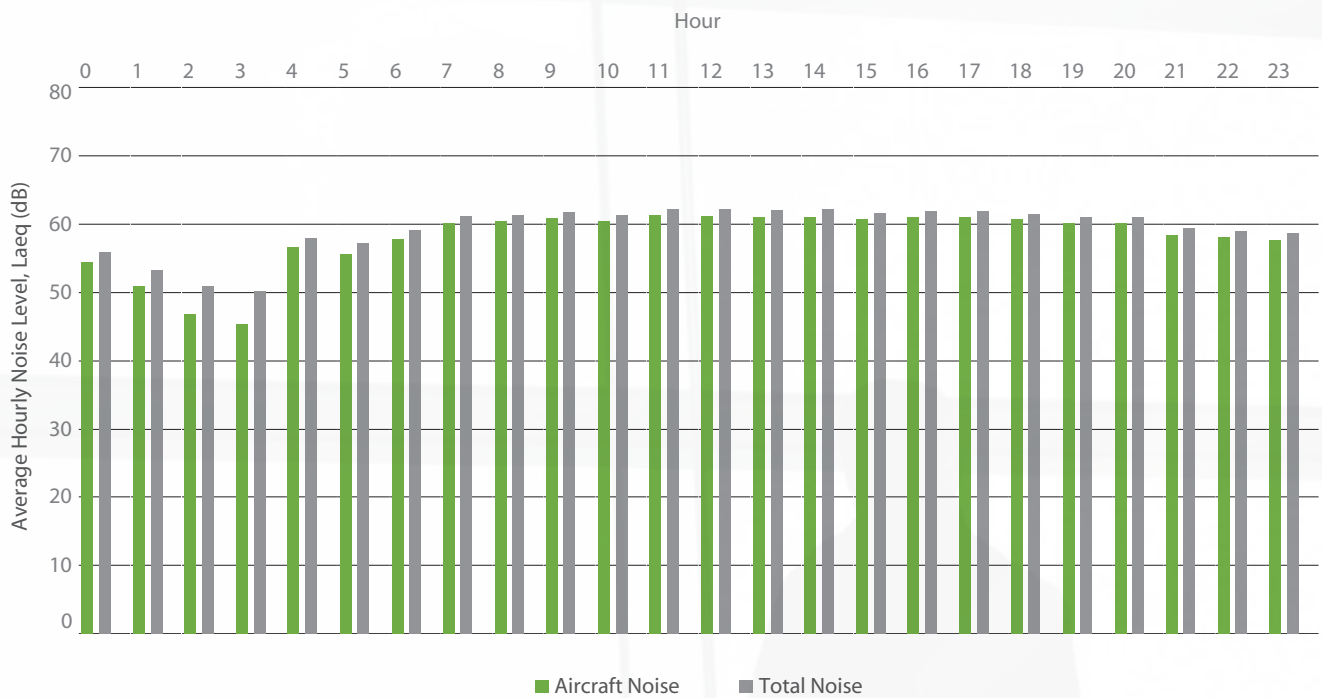
Figure 18: Averaged hourly noise levels for NMT 2, January - June 2018
