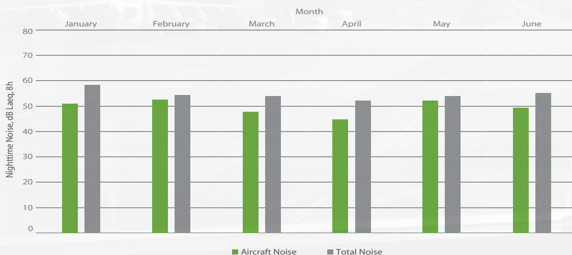
Figure 31: Averaged nighttime noise levels for NMT 5, January - June 2018
