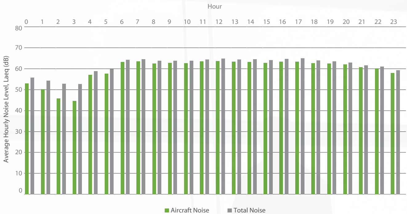
Figure 11: Averaged hourly noise levels for NMT 1, January - June 2018
