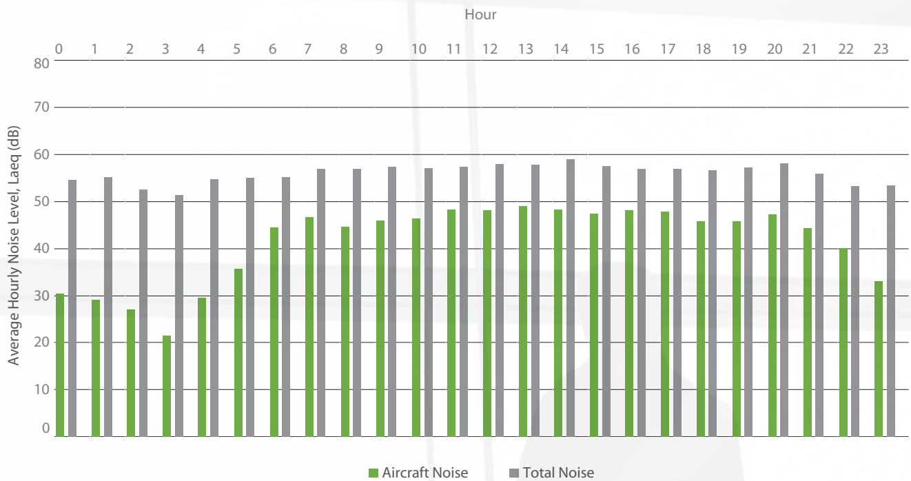
Figure 25: Averaged hourly noise levels for NMT 4, January - June 2018
