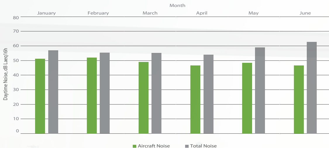
Figure 30: Averaged daytime noise levels for NMT 5, January - June 2018
