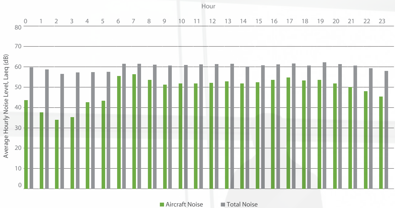
Figure 53: Averaged hourly noise levels for NMT 21, January - June 2018
