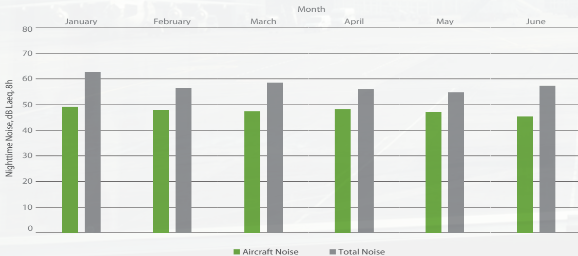
Figure 52: Averaged nighttime noise levels for NMT 21, January - June 2018
