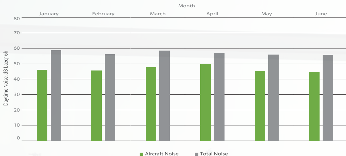
Figure 23: Averaged daytime noise levels for NMT 4, January - June 2018
