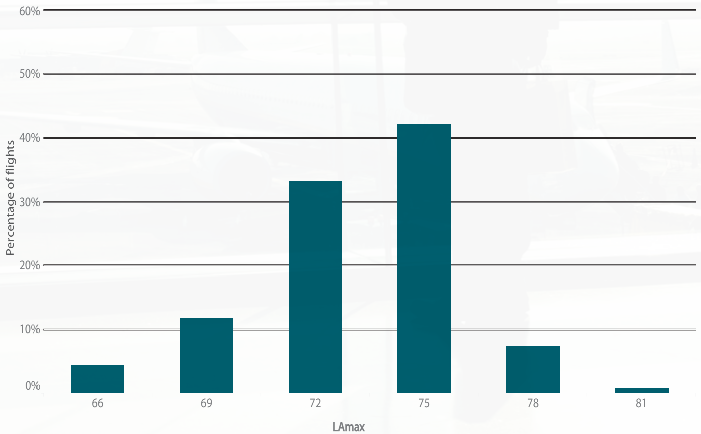
Figure 19: L_{A,MAX} levels distribution for NMT 2, January - June 2018
