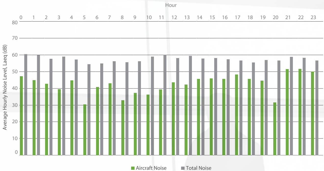
Figure 39: Averaged hourly noise levels for NMT 6, January - June 2018
