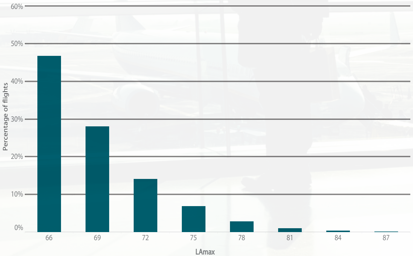
Figure 54: L_{A,MAX} levels distribution for NMT 21, January - June 2018
