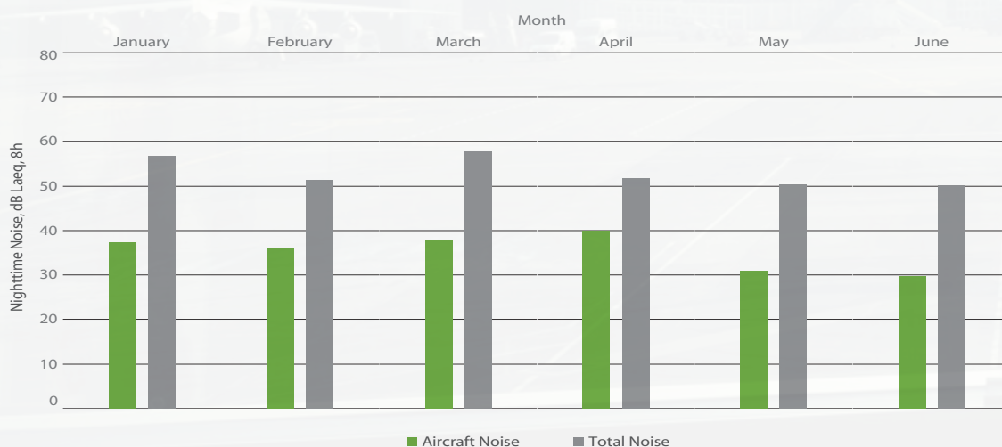
Figure 24: Averaged nighttime noise levels for NMT 4, January - June 2018
