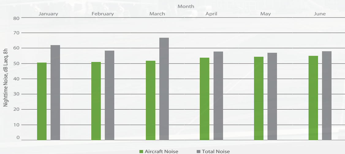
Figure 45: Averaged nighttime noise levels for NMT 20, January - June 2018
