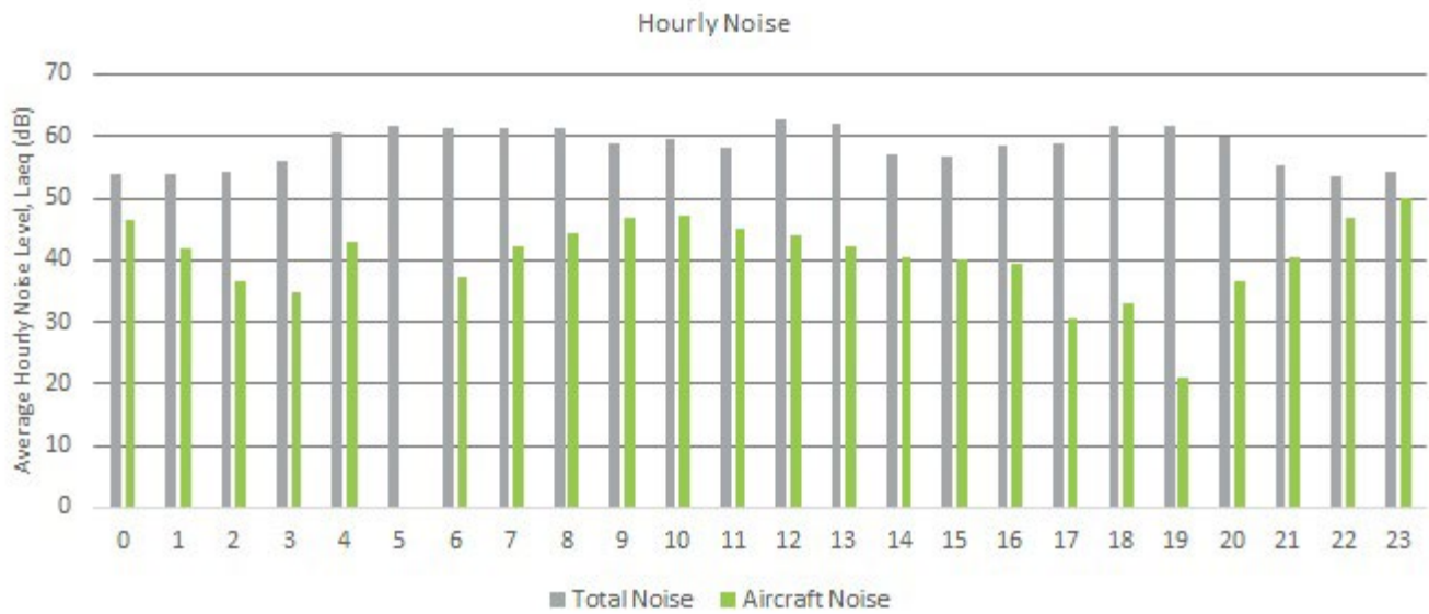
Figure 43: Averaged hourly noise levels for NMT 5, January- June 2022
