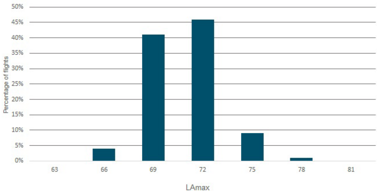
Figure 58: L Amax levels distribution for NMT 20, January- June 2022
