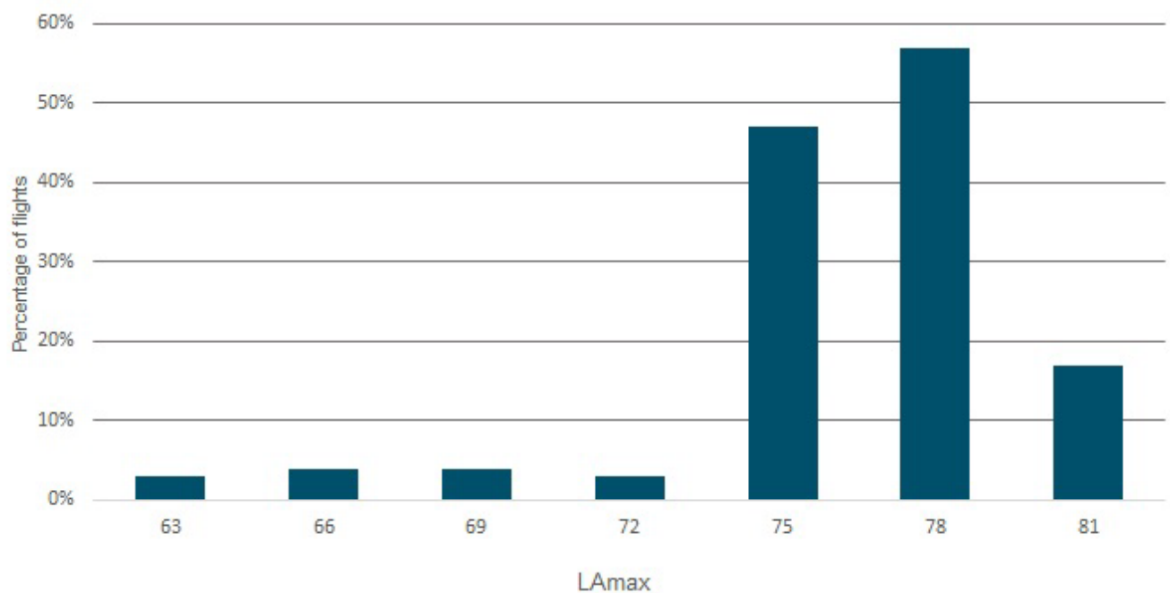
Figure 44: L_{Amax} levels distribution for NMT 5, January- June 2022
