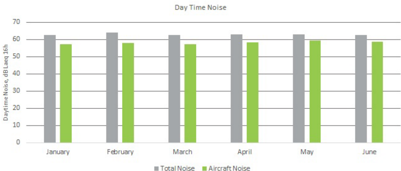
Figure 55: Averaged daytime noise levels for NMT 20, January- June 2022
