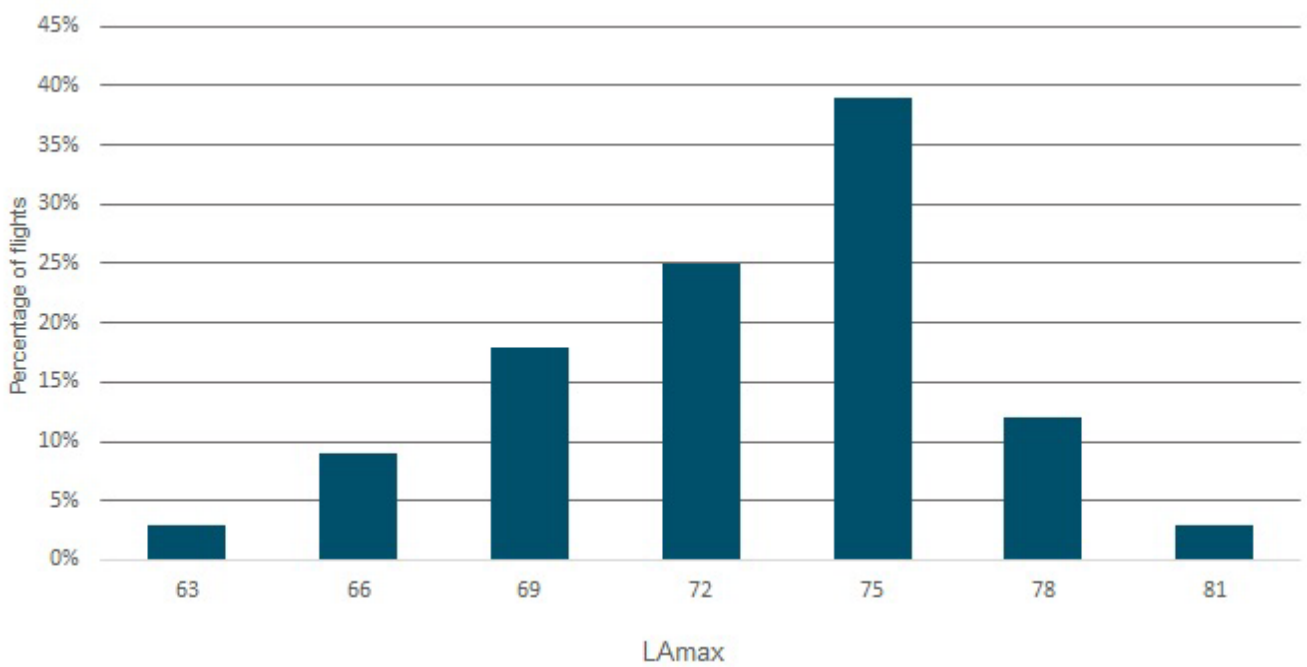
Figure 51: LAmax levels distribution for NMT 6, January- June 2022
