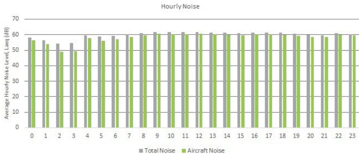
Figure 22: Averaged hourly noise levels for NMT 2, January- June 2022
