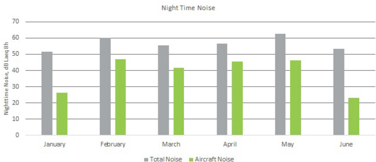
Figure 42: Averaged nighttime noise levels for NMT 5, January- June 2022
