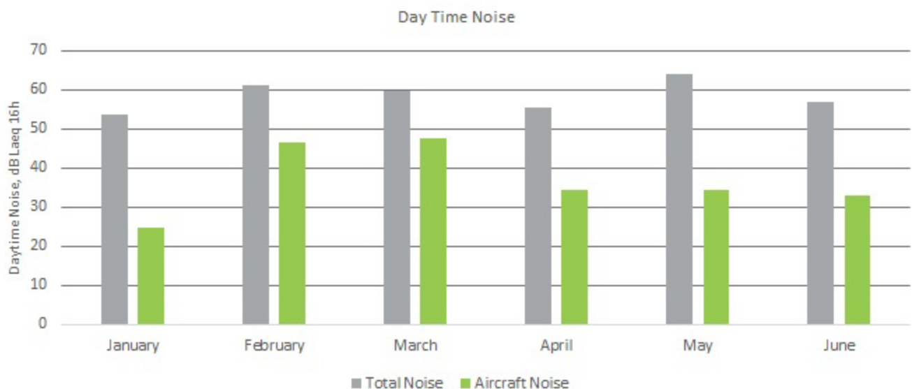
Figure 41: Averaged daytime noise levels for NMT 5, January- June 2022
