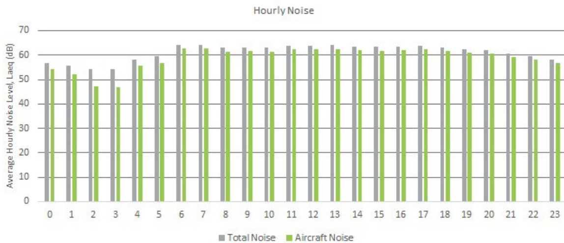
Figure 15: Averaged hourly noise levels for NMT 1, January- June 2022
