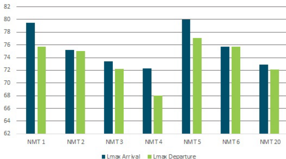
Figure 7: Average LAmax levels distribution for NMTs for arriving and departing aircraft, January – June 2022
