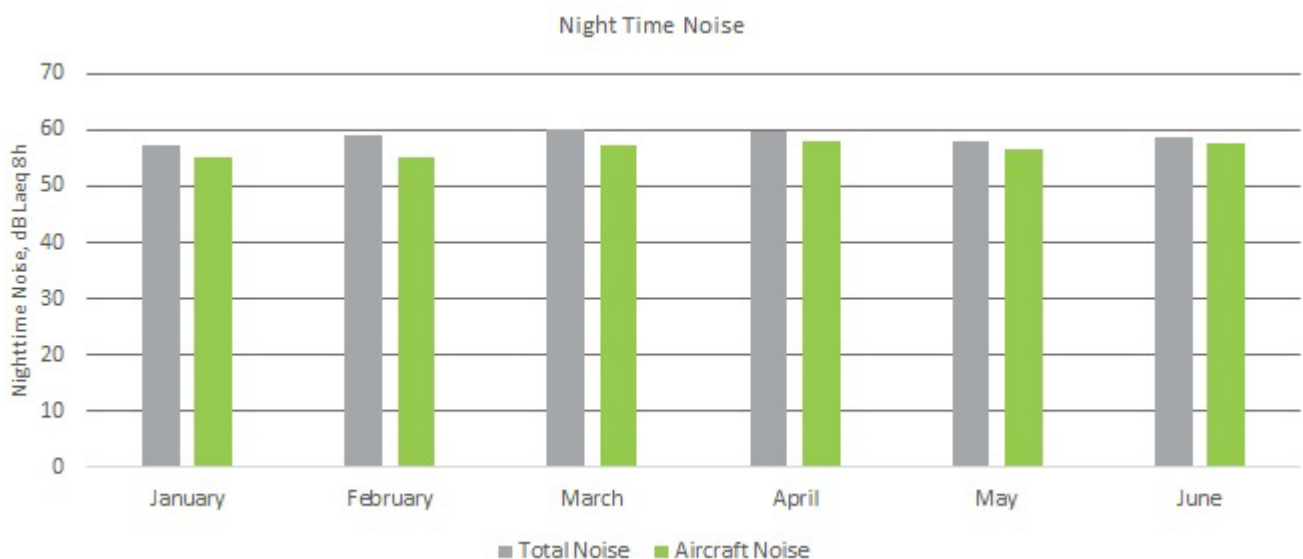
Figure 14: Averaged nighttime noise levels for NMT 1, January- June 2022
