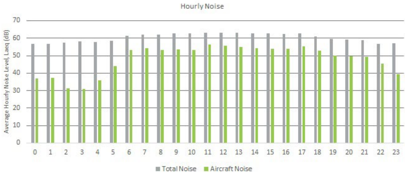
Figure 29: Averaged hourly noise levels for NMT 3, January- June 2022
