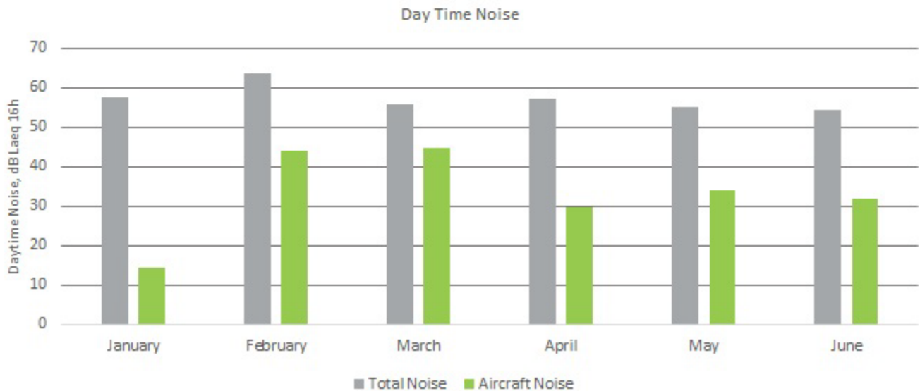
Figure 48: Averaged daytime noise levels for NMT 6, January- June 2022
