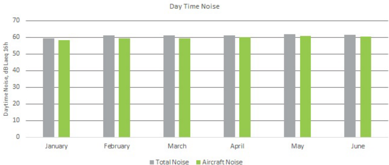
Figure 20: Averaged daytime noise levels for NMT 2, January- June 2022
