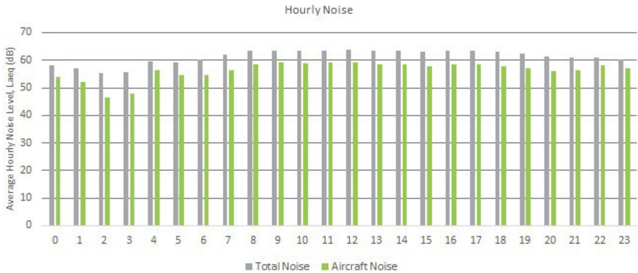
Figure 57: Averaged hourly noise levels for NMT 20, January- June 2022
