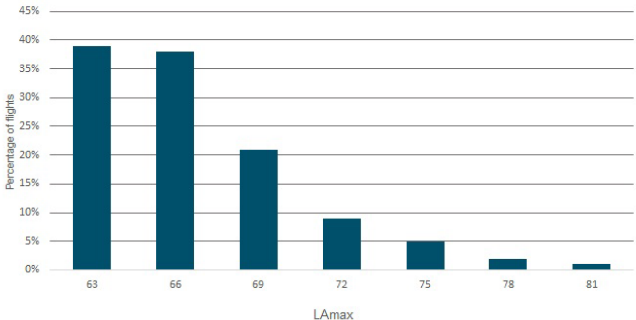
Figure 37: LAmax levels distribution for NMT 4, January- June 2022
