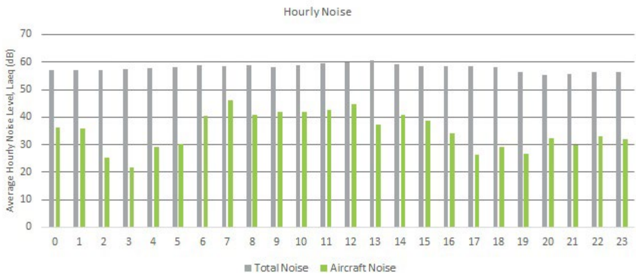
Figure 50: Averaged hourly noise levels for NMT 6, January- June 2022
