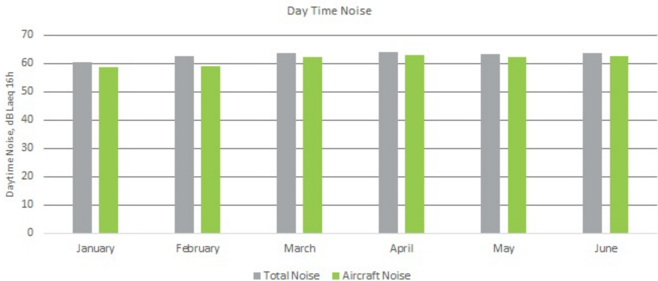
Figure 13: Averaged daytime noise levels for NMT 1, January- June 2022
