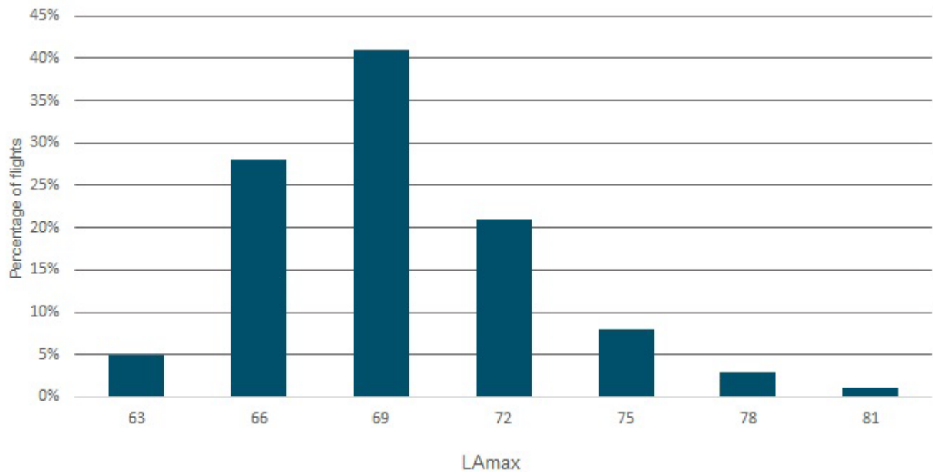
Figure 30: L Amax levels distribution for NMT 3, January- June 2022
