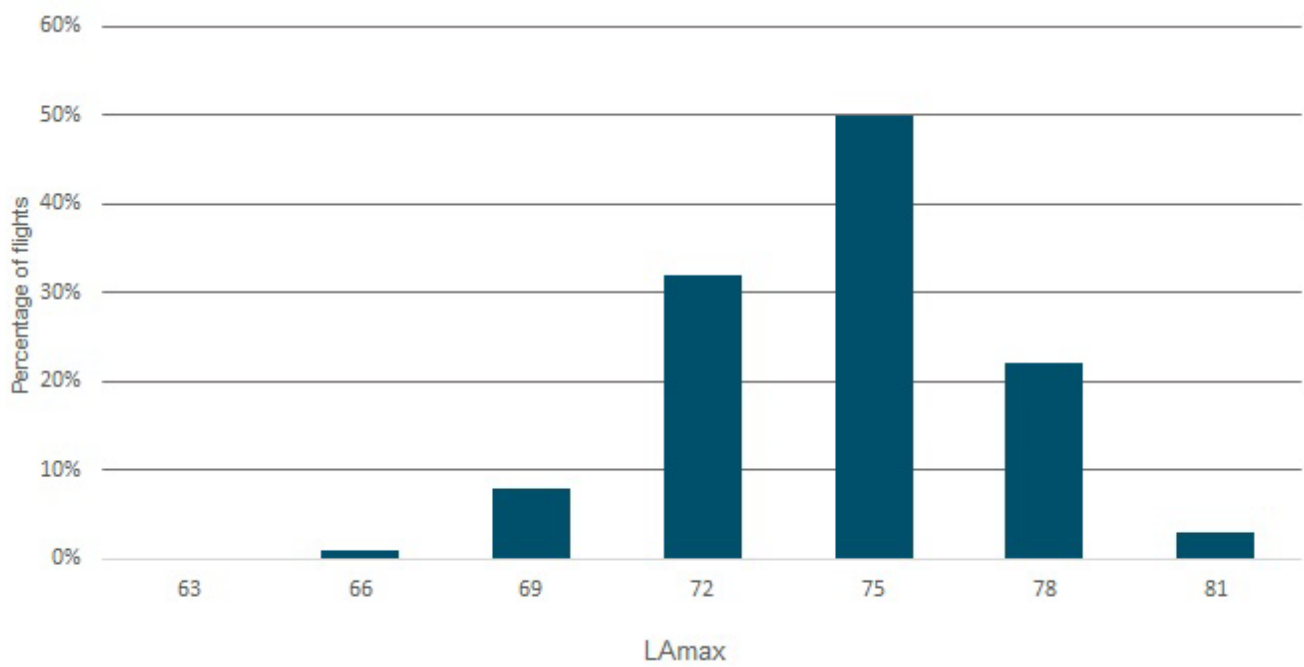
Figure 16: LAmax levels distribution for NMT 1, January- June 2022
