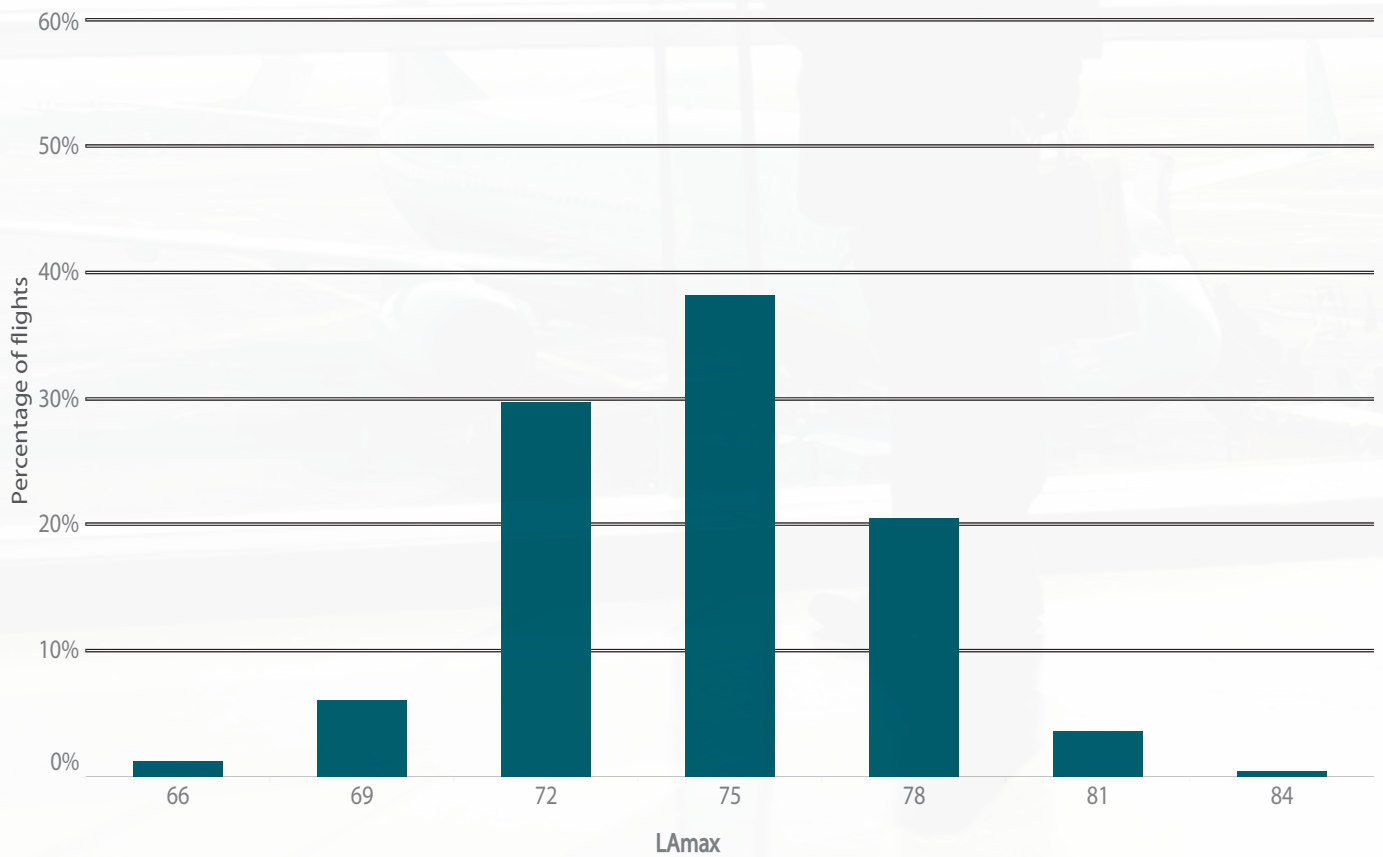
Figure 12: L_{A,MAX} levels distribution for NMT 1, July – December 2018
