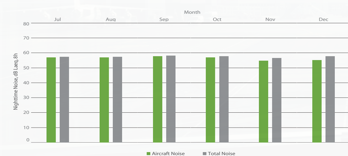
Figure 17: Averaged nighttime noise levels for NMT 2, July – December 2018
