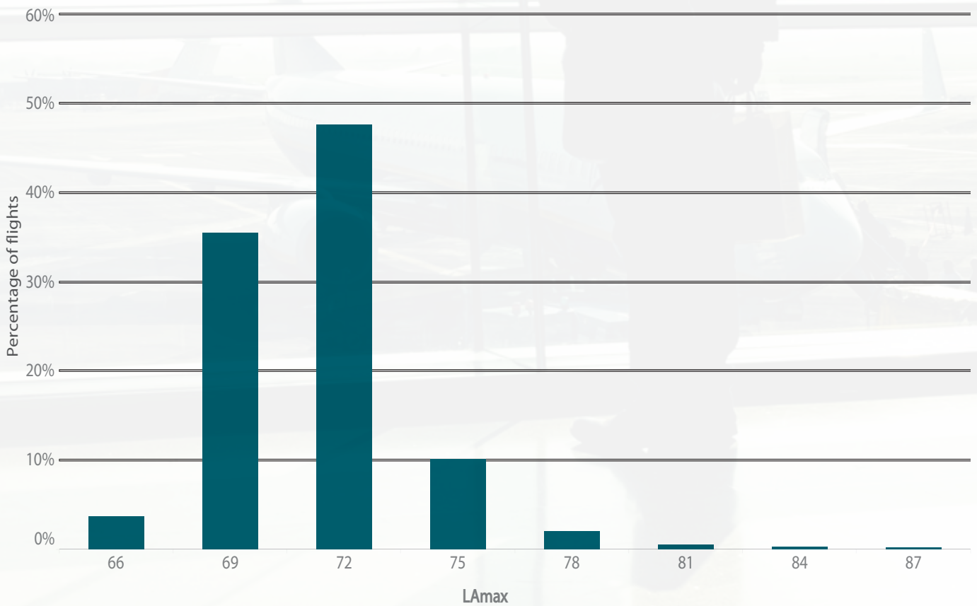
Figure 47: L_{A,MAX} levels distribution for NMT 20, July – December 2018
