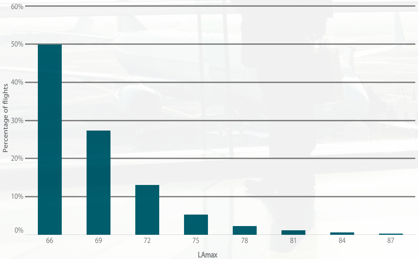
Figure 54: L_{A,MAX} levels distribution for NMT 21, July – December 2018
