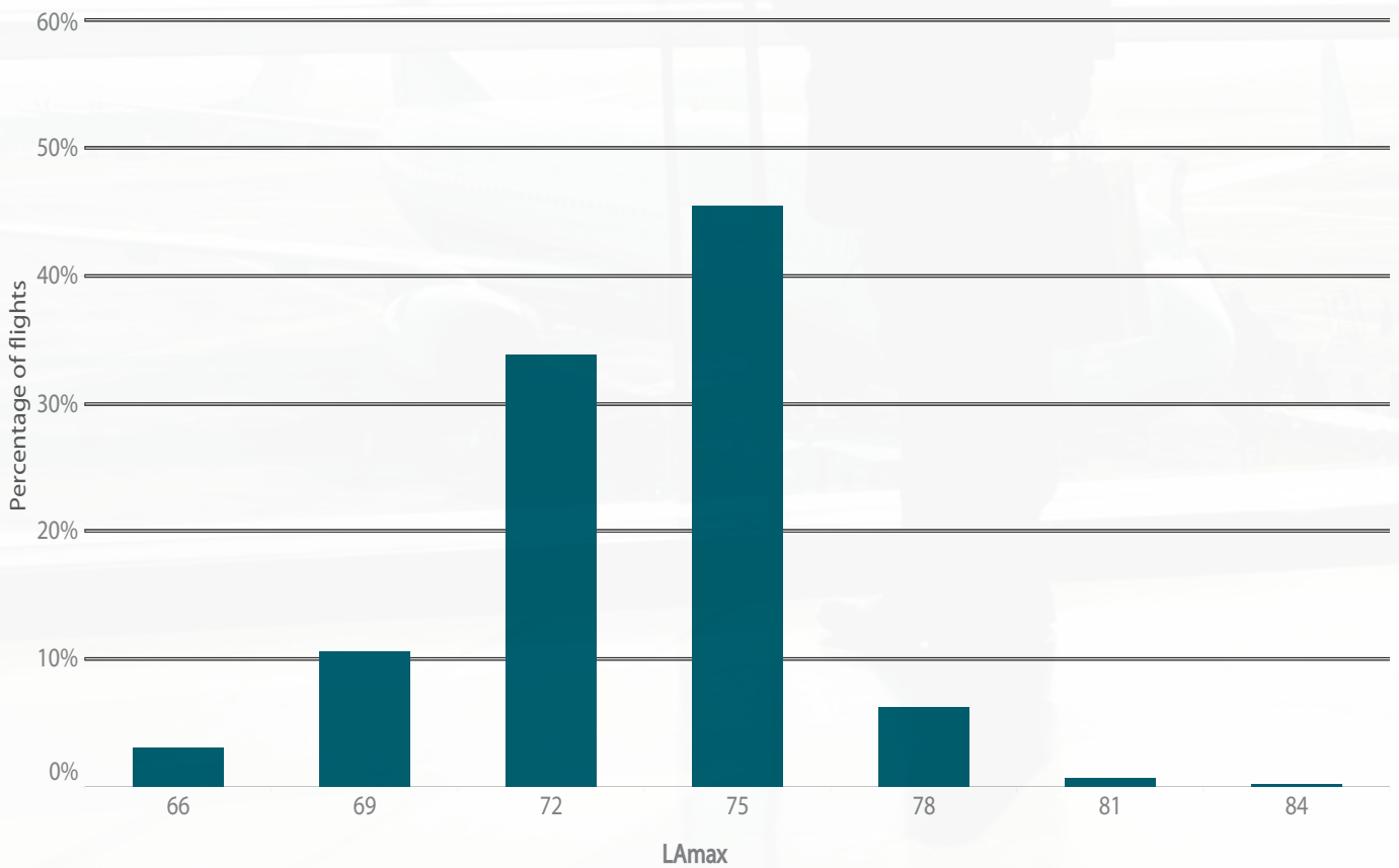
Figure 19: L_{A,MAX} levels distribution for NMT 2, July – December 2018
