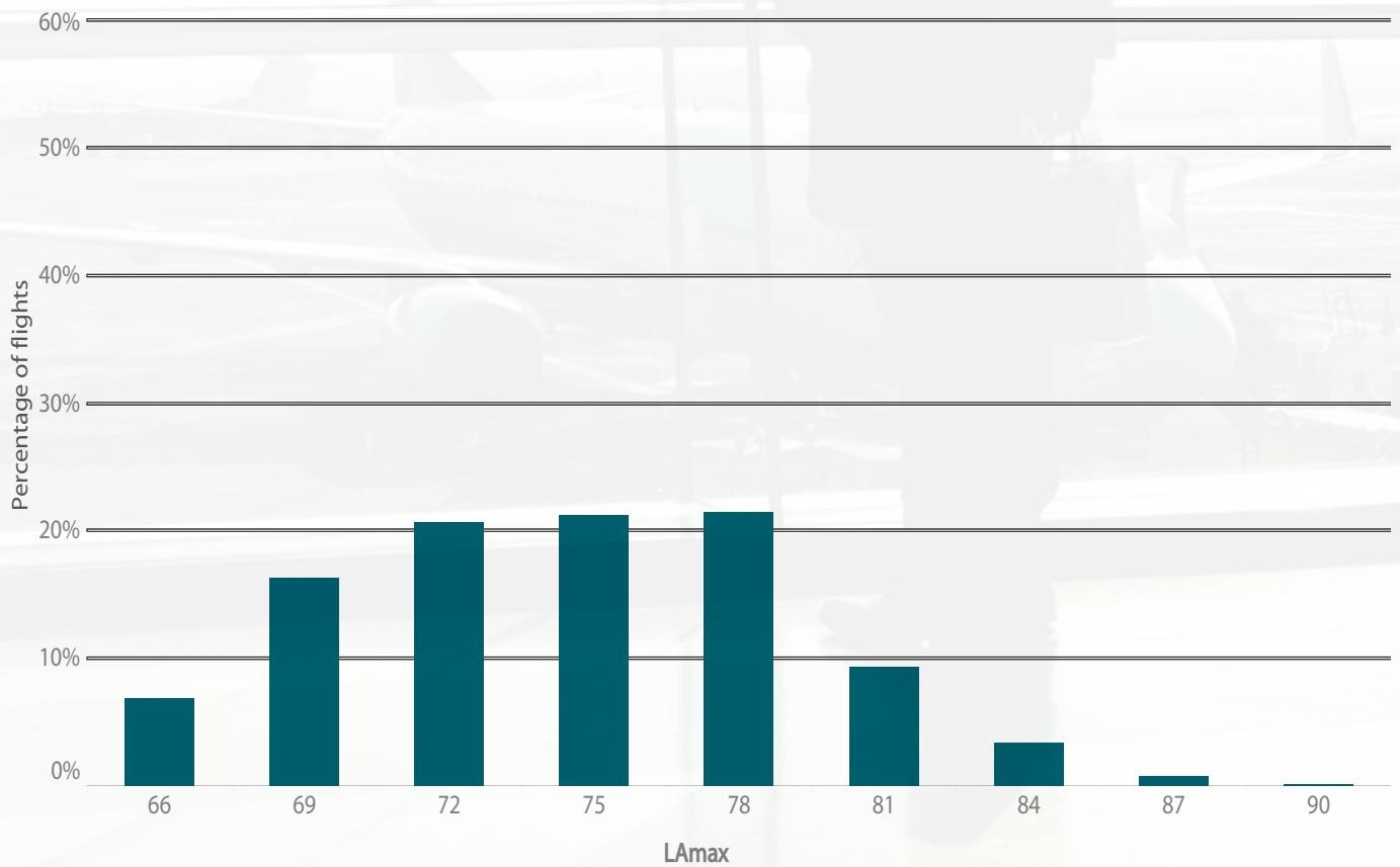
Figure 33: L_{A,MAX} levels distribution for NMT 5, July – December 2018
