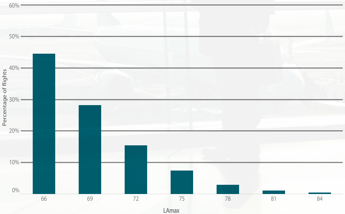
Figure 26: L_{A,MAX} levels distribution for NMT 4, July – December 2018
