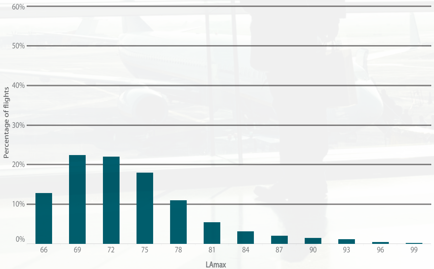
Figure 40: L_{A,MAX} levels distribution for NMT 6, July – December 2018
